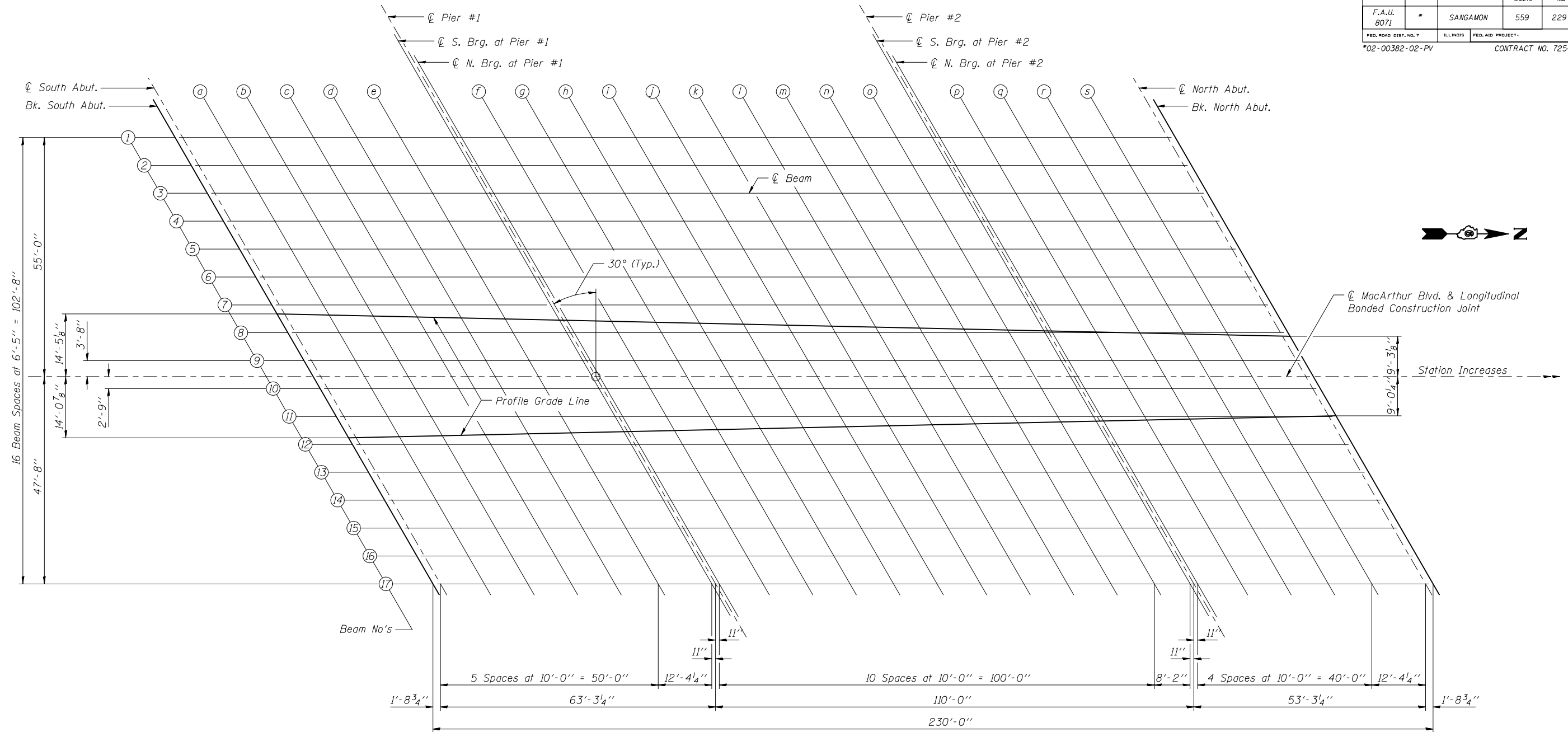
DIAGRAMMATIC PLAN
