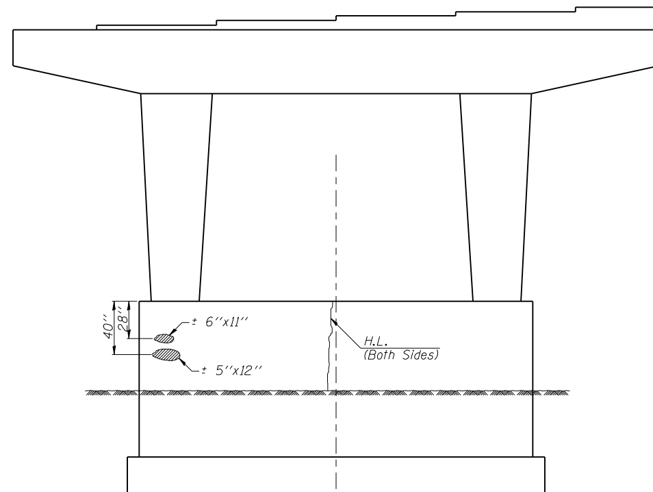
PIER 2 I-72 E.B. (Looking East)
