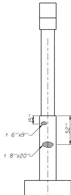
END VIEW - PIER 2 (I-72 E.B. North Side)
