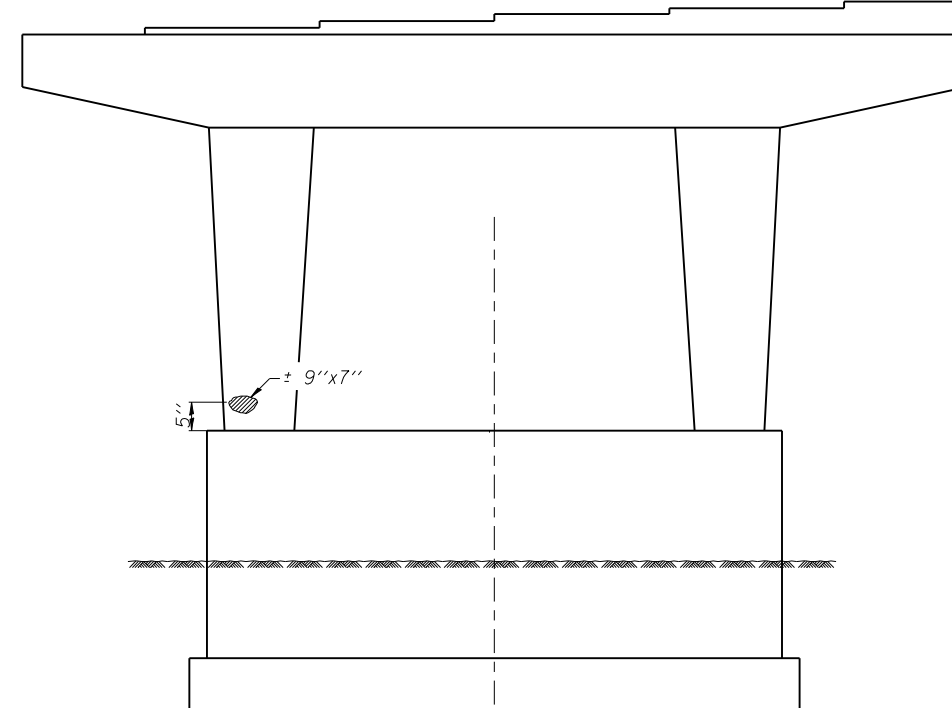
PIER 2 I-72 W.B. (Looking East)
