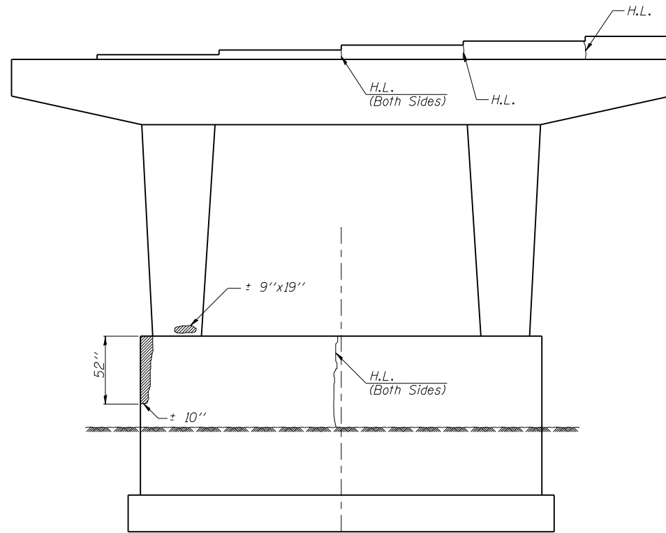
PIER 1 I-72 E.B. (Looking East)
