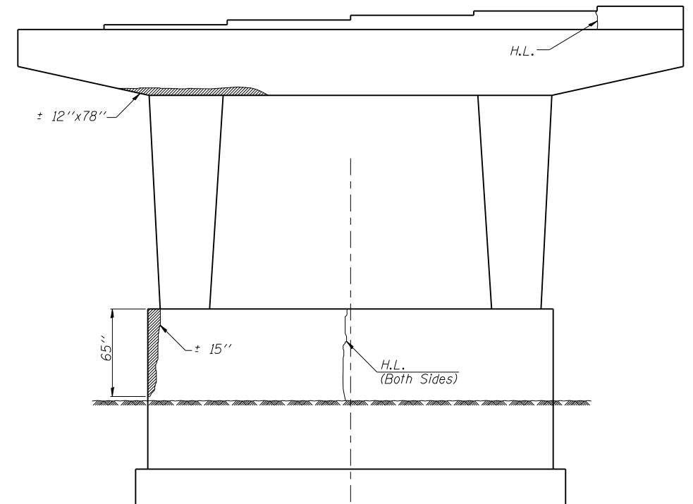
PIER 1 I-72 W.B. (Looking East)
