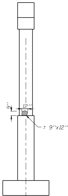
END VIEW - PIER 1 (I-72 E.B. South Side)
