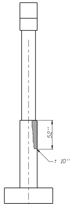
END VIEW - PIER 1 (I-72 E.B. North Side)
