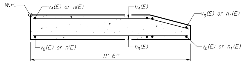
SEC. B-B
