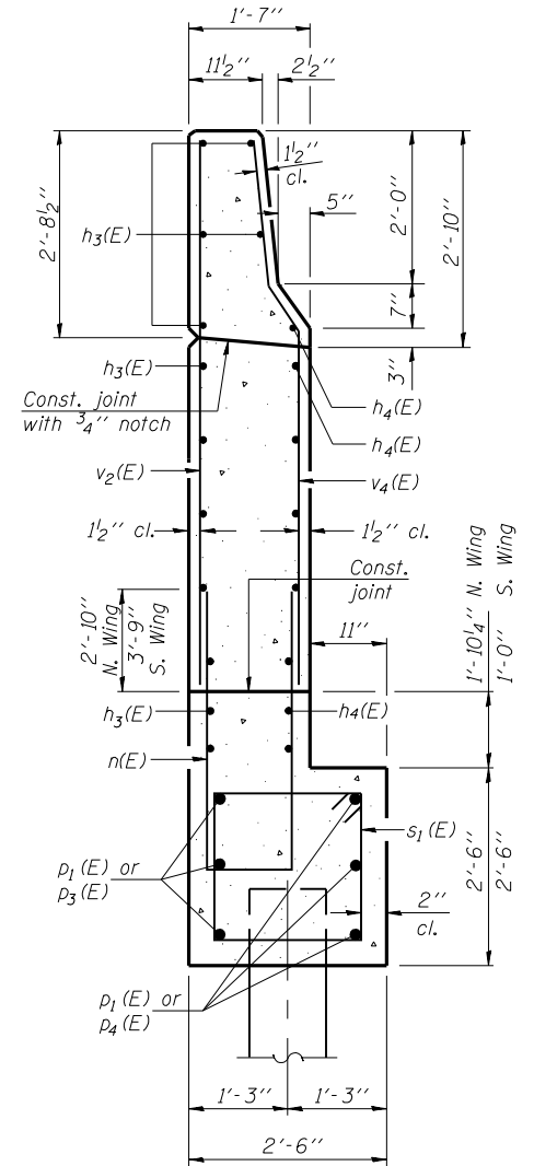
SECTION C-C
