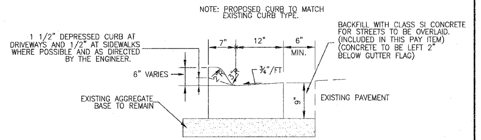
DETAIL OF COMBINATION CONCRETE CURB & GUTTER REMOVAL & REPLACEMENT NO SCALE
