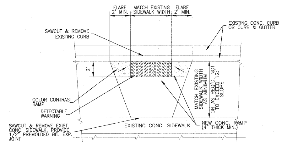
DETECTABLE WARNINGS DETAIL NO SCALE
