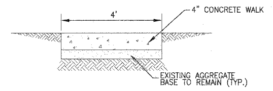
NOTE: PROVIDE FIBER 3/4" EXPANSION JOINTS WHERE NEW SIDEWALK MEETS EXISTING AND @ 48' O.C. MAX. AND PROVIDE CONTROL JOINTS @ 4' O.C. PORTLAND CEMENT CONCRETE (P.C.C.) SIDEWALK - 4-INCH NO SCALE
