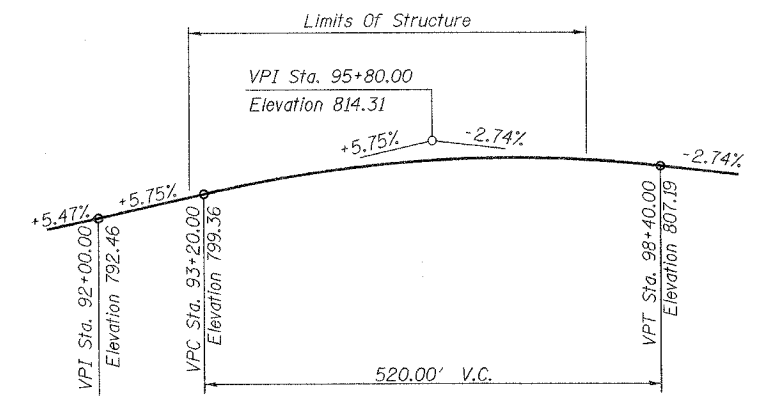
PROFILE GRADE
