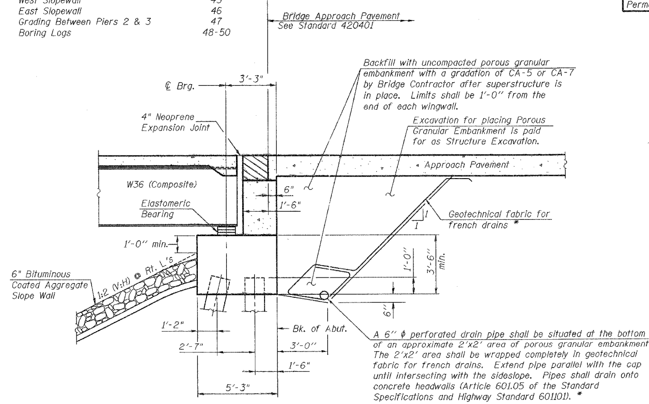
SECTION THRU ABUTMENT (Horiz. dim. @ Rt. L's)
