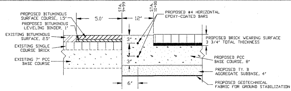
CONCRETE HEADER DETAIL SOUTH END PROJECT STATION 9+99 - 10+00
