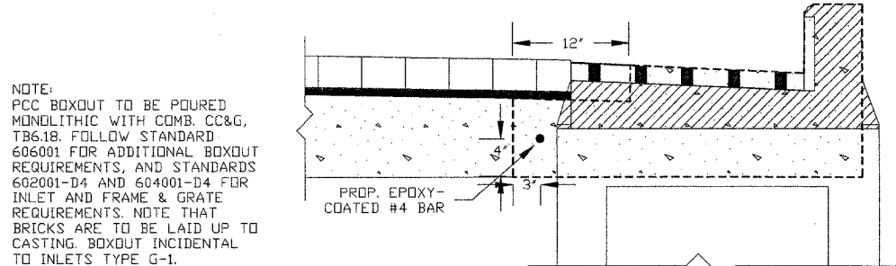
INLET TG-1 DETAIL SECTION A-A STATIONS 28+30 R&L
