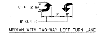
TYPICAL PAINTED MEDIAN MARKING
