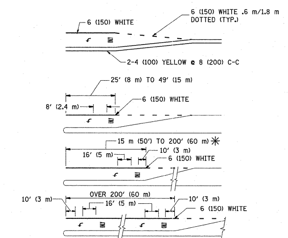
TYPICAL PAINTED MEDIAN MARKING
