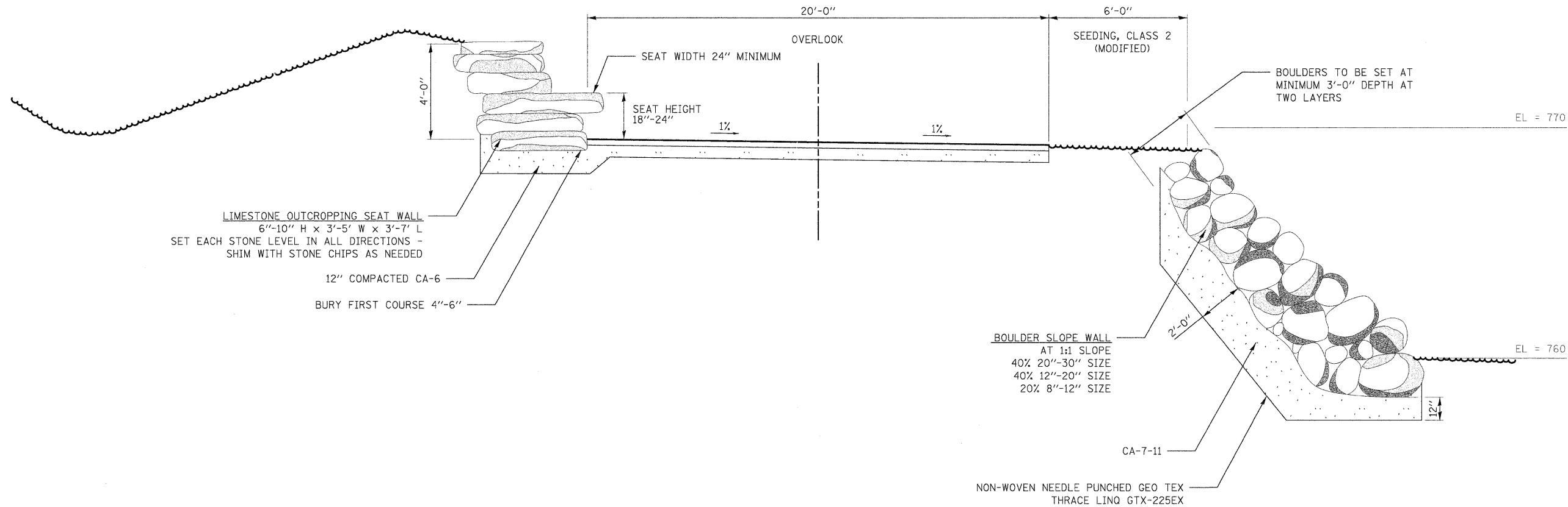
OVERLOOK DETAIL
