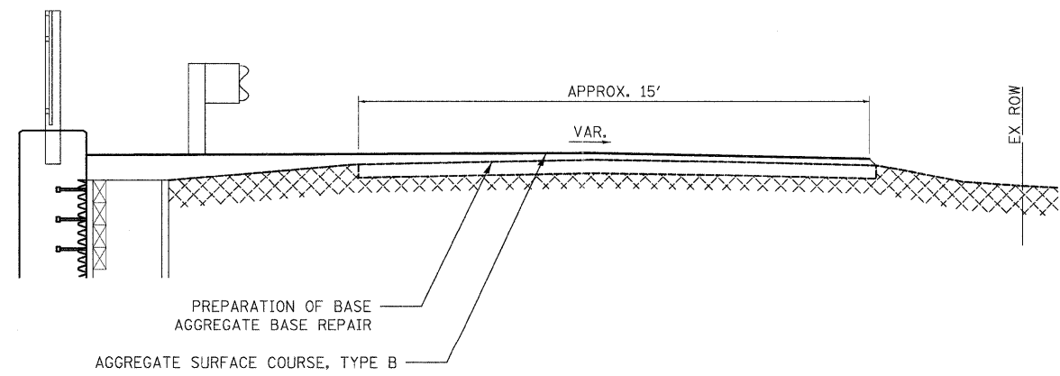
AGGREGATE DRIVEWAY SECTION
