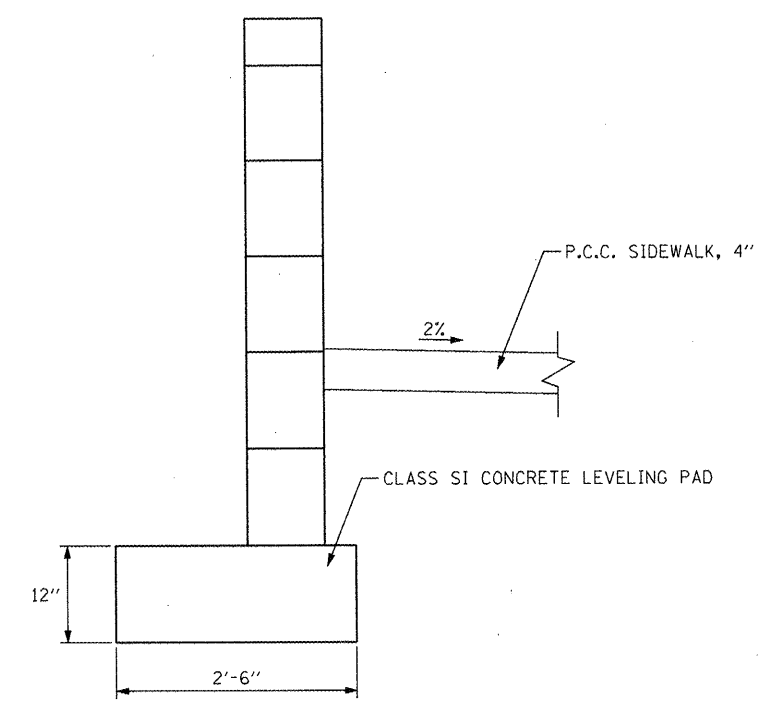
WALL SECTION (LOOKING UPSTATION)
