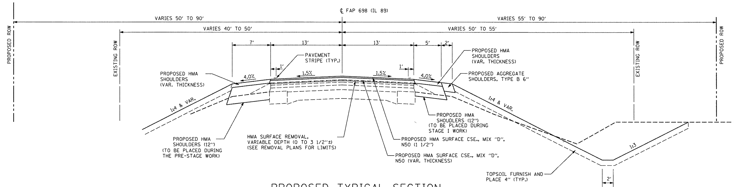
PROPOSED TYPICAL SECTION STA. 193+11 TO STA. 206+24
