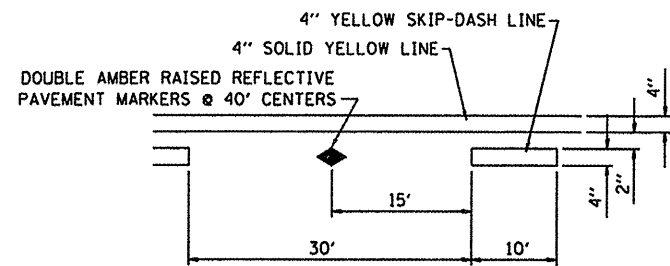
TYPICAL APPLICATION FOR SOLID YELLOW, SKIP-DASH LANE LINES WITH RAISED REFLECTIVE PAVEMENT MARKERS SOLID YELLOW, SKIP DASH PAVEMENT MARKING DETAIL (NOT TO SCALE)
