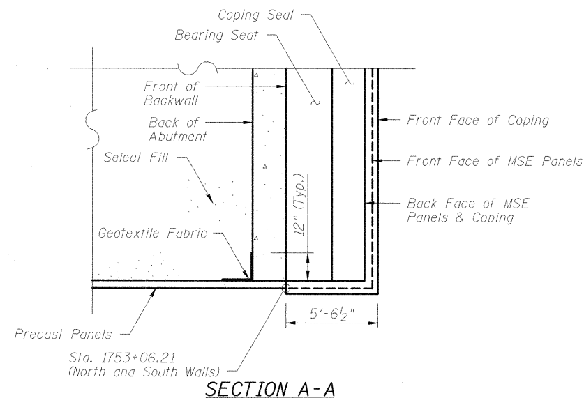
WRAP AROUND WALL DETAILS
