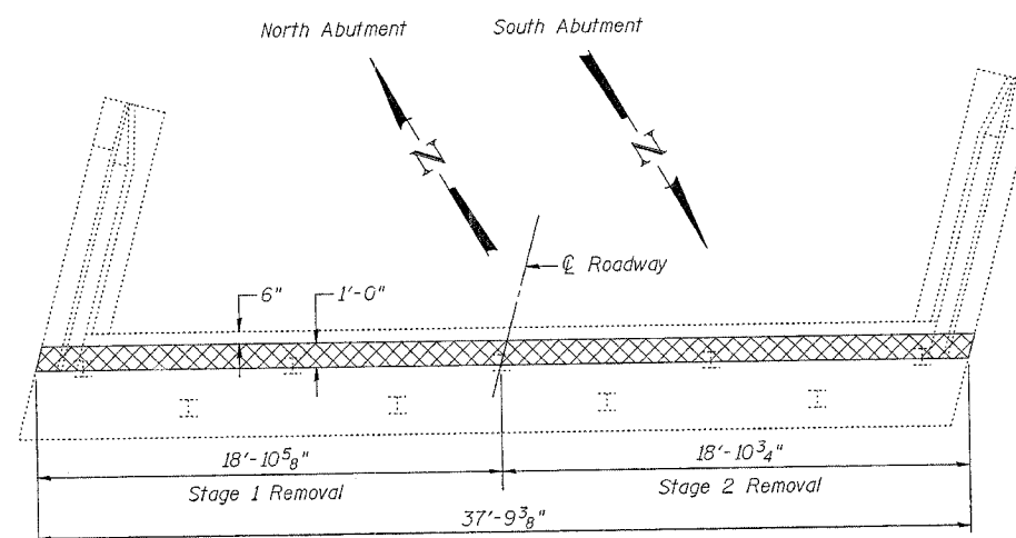
ABUTMENT PLAN
