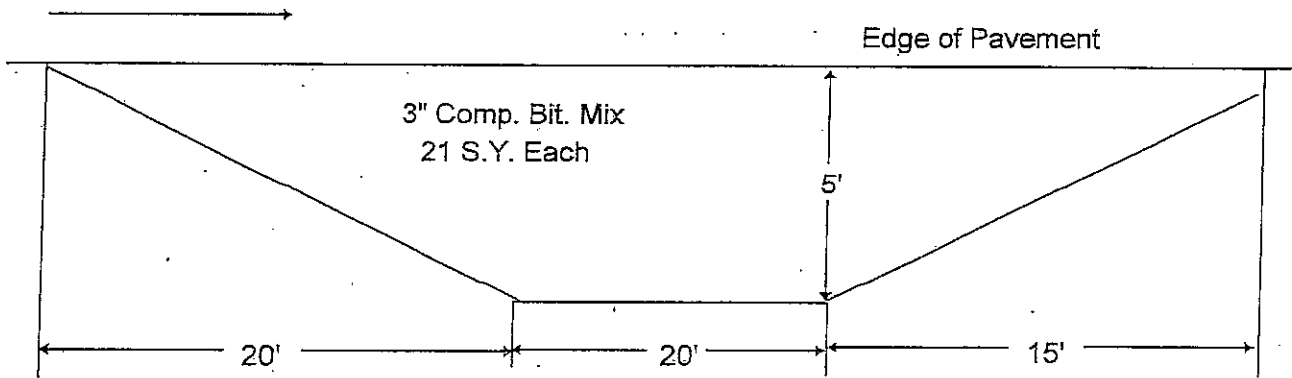
TYPICAL PRIVATE ENTRANCE
