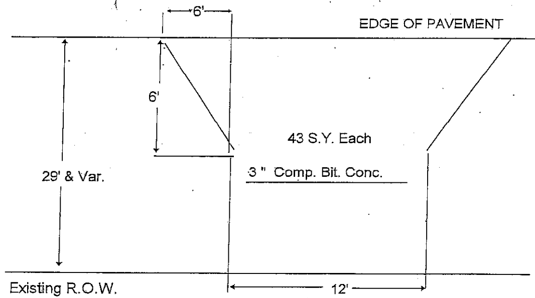
TYPICAL PRIVATE ENTRANCE
