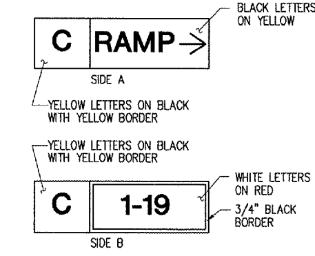
TAXIWAY GUIDANCE SIGN TS-4 DETAIL "NOT TO SCALE"
