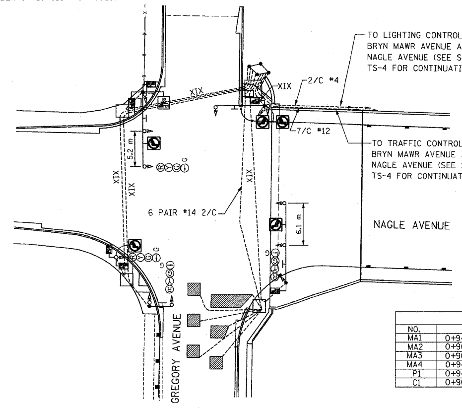
SIGNAL AND CABLE PLAN NOT TO SCALE
