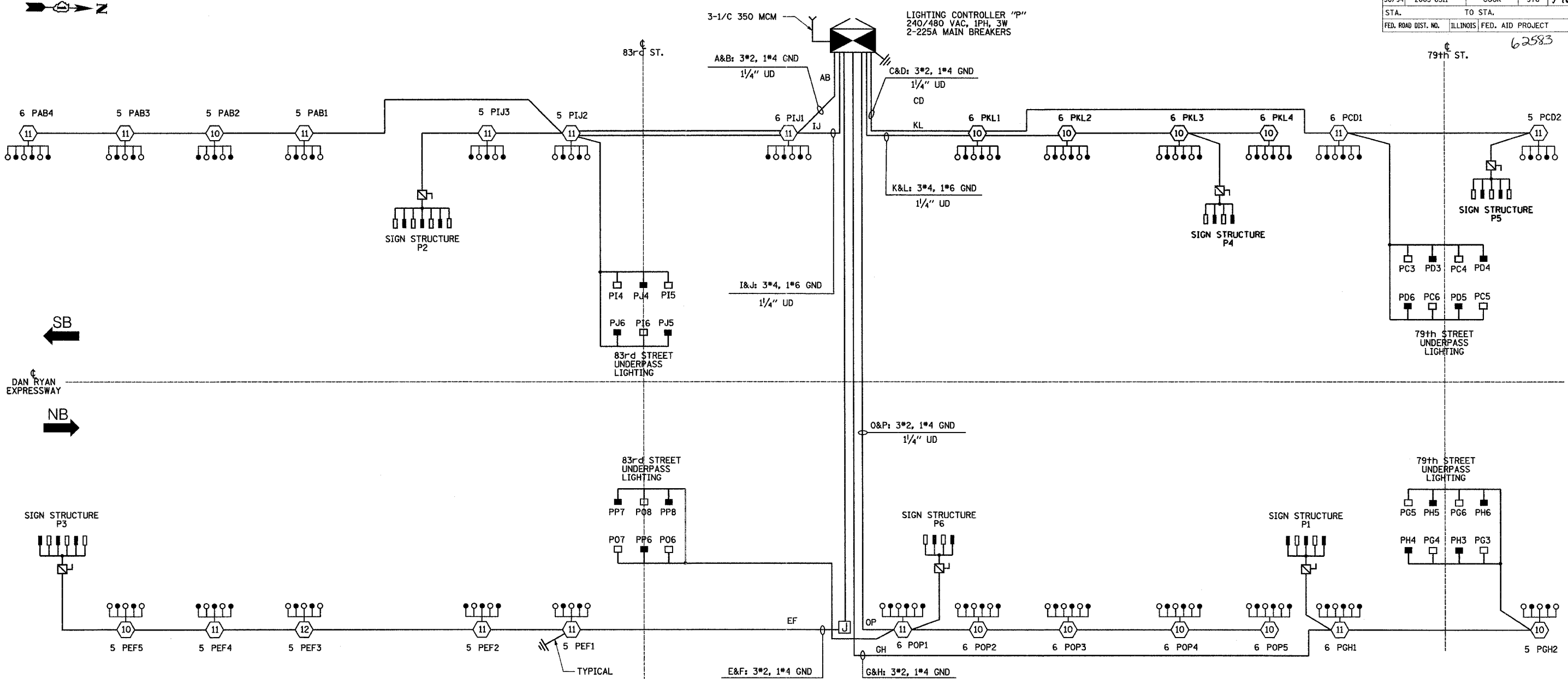
SINGLE LINE DIAGRAM LIGHTING CONTROLLER "P"
