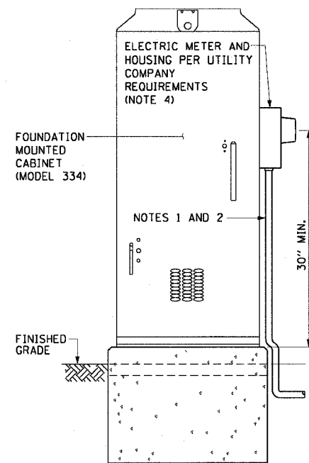
UPS CABINET FRONT VIEW (MODEL 334)
