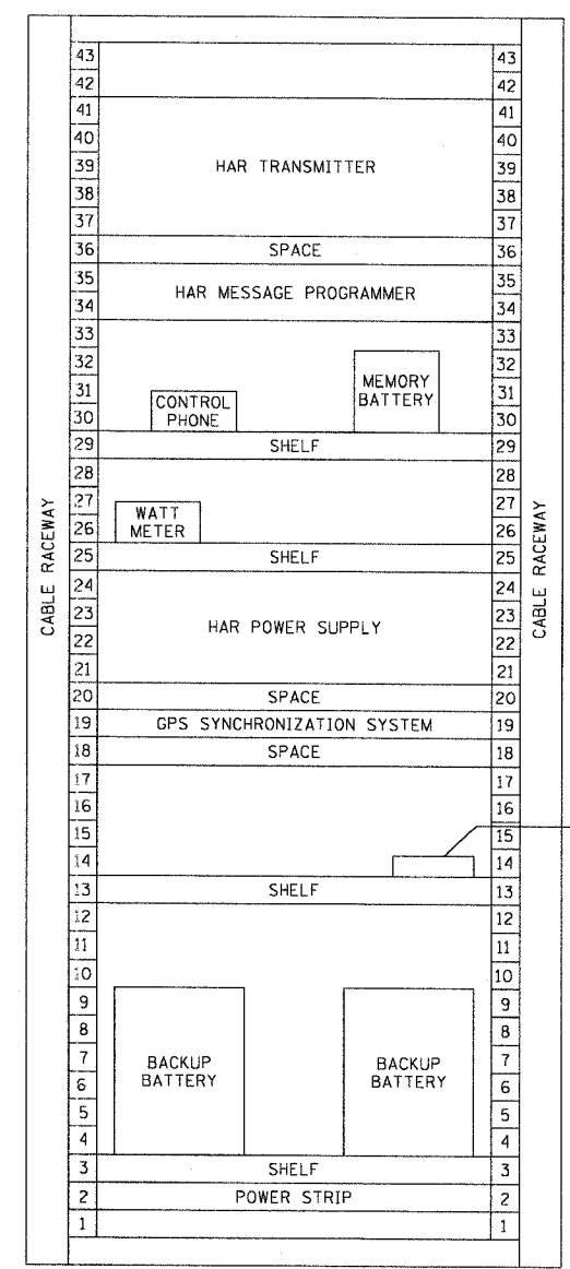
2 RACK LAYOUT 01-20 NOTES 2 AND 3 NOT TO SCALE
