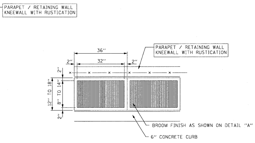
DETAIL "B" CALIFORNIA FINISH
