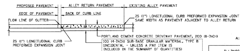
ALLEY RETURN DETAIL
