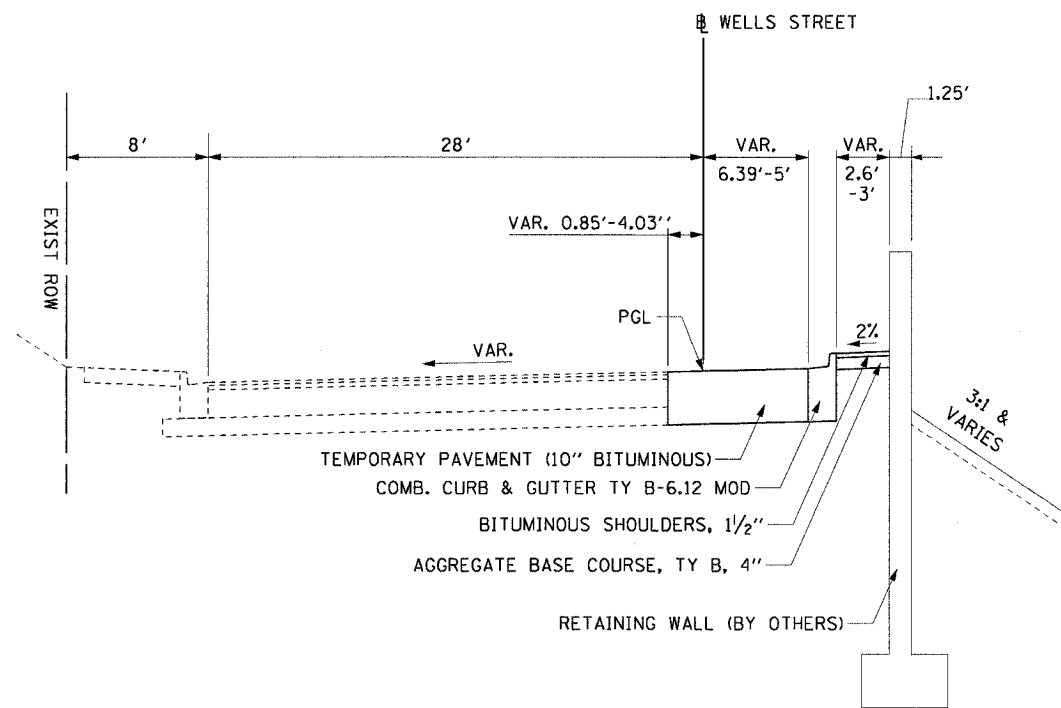
TEMPORARY PAVEMENT DETAIL STA 534+83.41 TO STA 535+32.53
