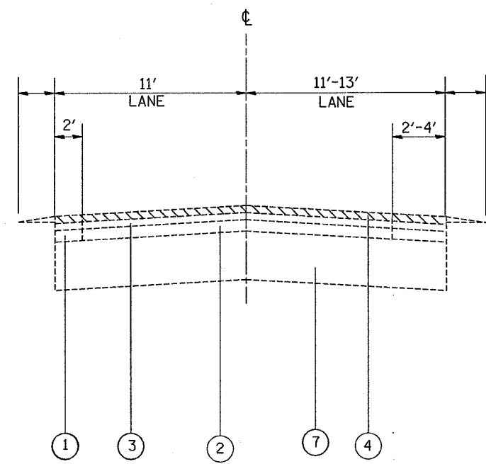
EXISTING TYPICAL CROSS SECTION STA. 0+38 TO STA. 10+16 (LOOKING NORTHEAST)
