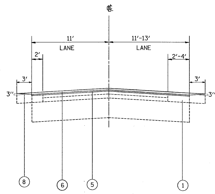
PROPOSED TYPICAL CROSS SECTION STA. 0+38 TO STA. 10+16 (LOOKING NORTHEAST)
