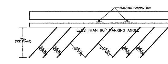
RESERVED PARKING SIGN DETAIL 44.2 REVISED 10-15-04
