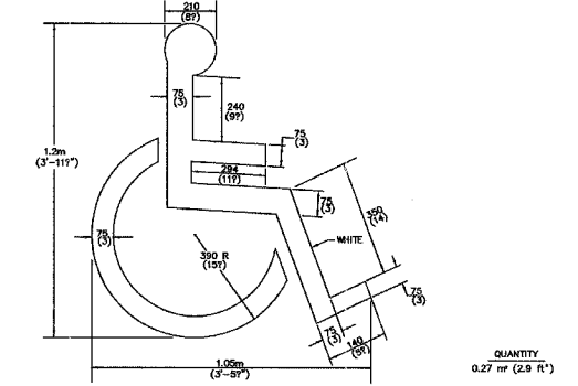
DISABLED SYMBOL 69.4 QUANTITY 0.27 sq (2.8 sq ft) REVISED 5-4-04
