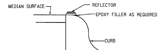
SECTION VIEW
