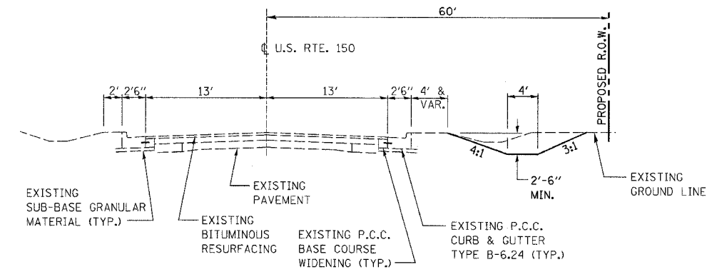
PROPOSED TYPICAL SECTION STA. 75+00 TO STA. 84+00 LOOKING EAST
