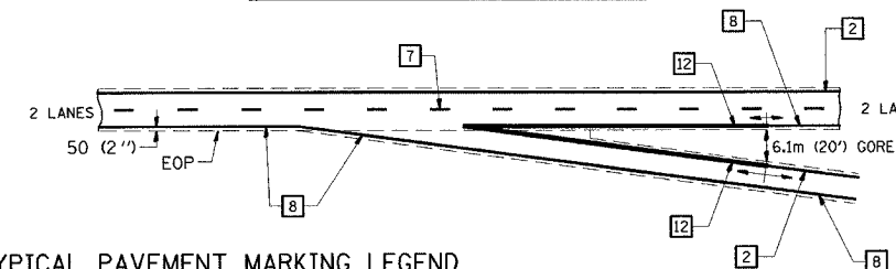
TYPICAL PAVEMENT MARKING LEGEND
