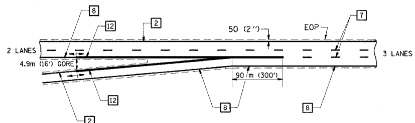
ENTRANCE RAMP TERMINAL with EXCLUSIVE LANE
