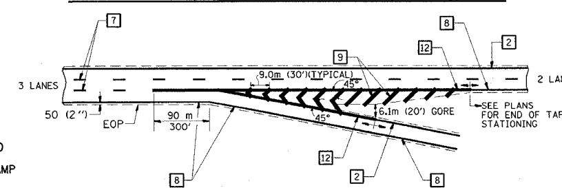
EXIT RAMP TERMINAL with EXCLUSIVE (auxiliary) LANE
