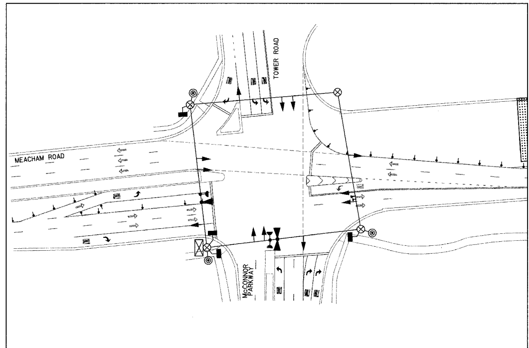
MAINTENANCE OF TRAFFIC STAGE III-A
