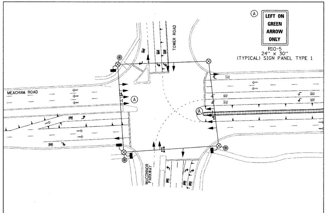
MAINTENANCE OF TRAFFIC STAGE IV
