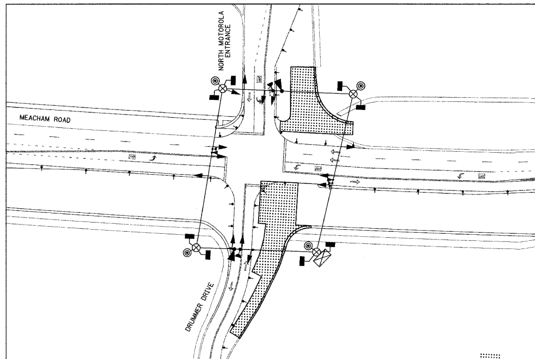
MAINTENANCE OF TRAFFIC STAGE II-C
