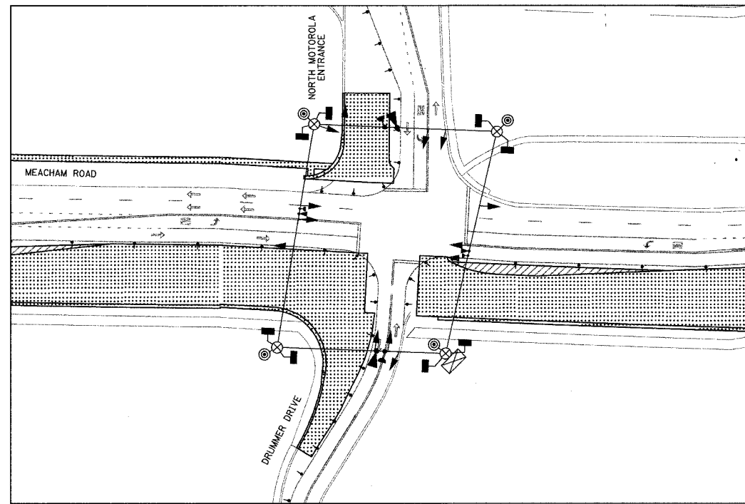
MAINTENANCE OF TRAFFIC STAGES II-A AND II-B
