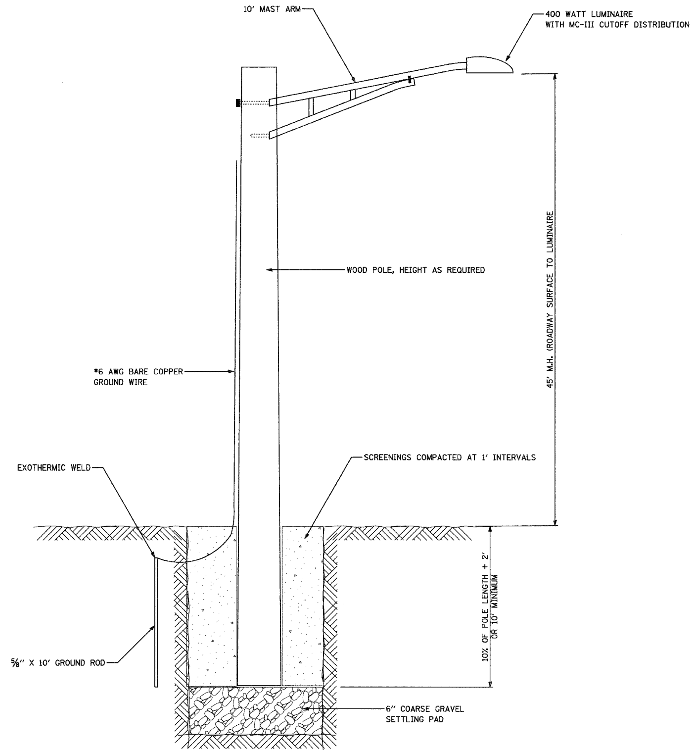
TEMPORARY WOOD LIGHT POLE DETAIL NOT TO SCALE
