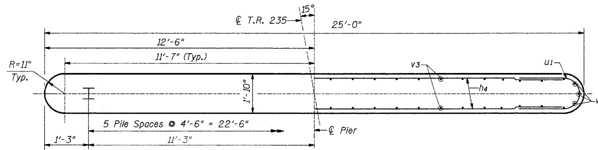
SECTION B-B
