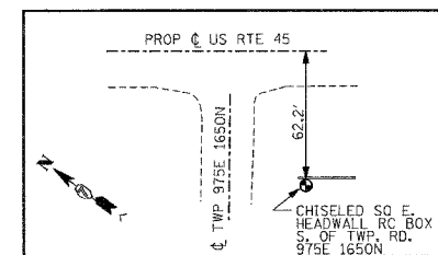
BENCHMARK #16 STA 1048+90 ELEVATION 487.81
