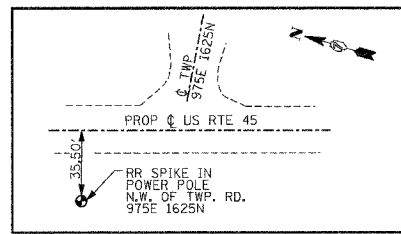
BENCHMARK #15 STA 1062+82 ELEVATION 507.60
