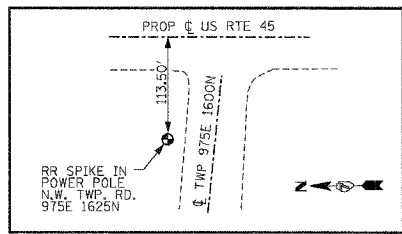
BENCHMARK #14 STA 1076+03 ELEVATION 507.41
