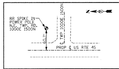
BENCHMARK #10 STA 1131+05 ELEVATION 501.86
