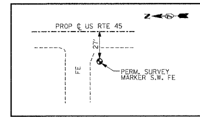
BENCHMARK #11 STA 1117+53.20 ELEVATION 499.34
