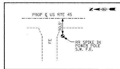
BENCHMARK #20 STA 992+84 ELEVATION 512.97
