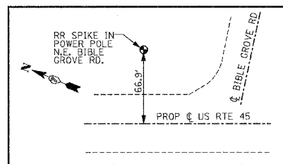
BENCHMARK #22 STA 964+50 ELEVATION 513.46
