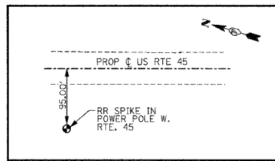
BENCHMARK #13 STA 1089+11 ELEVATION 500.06
