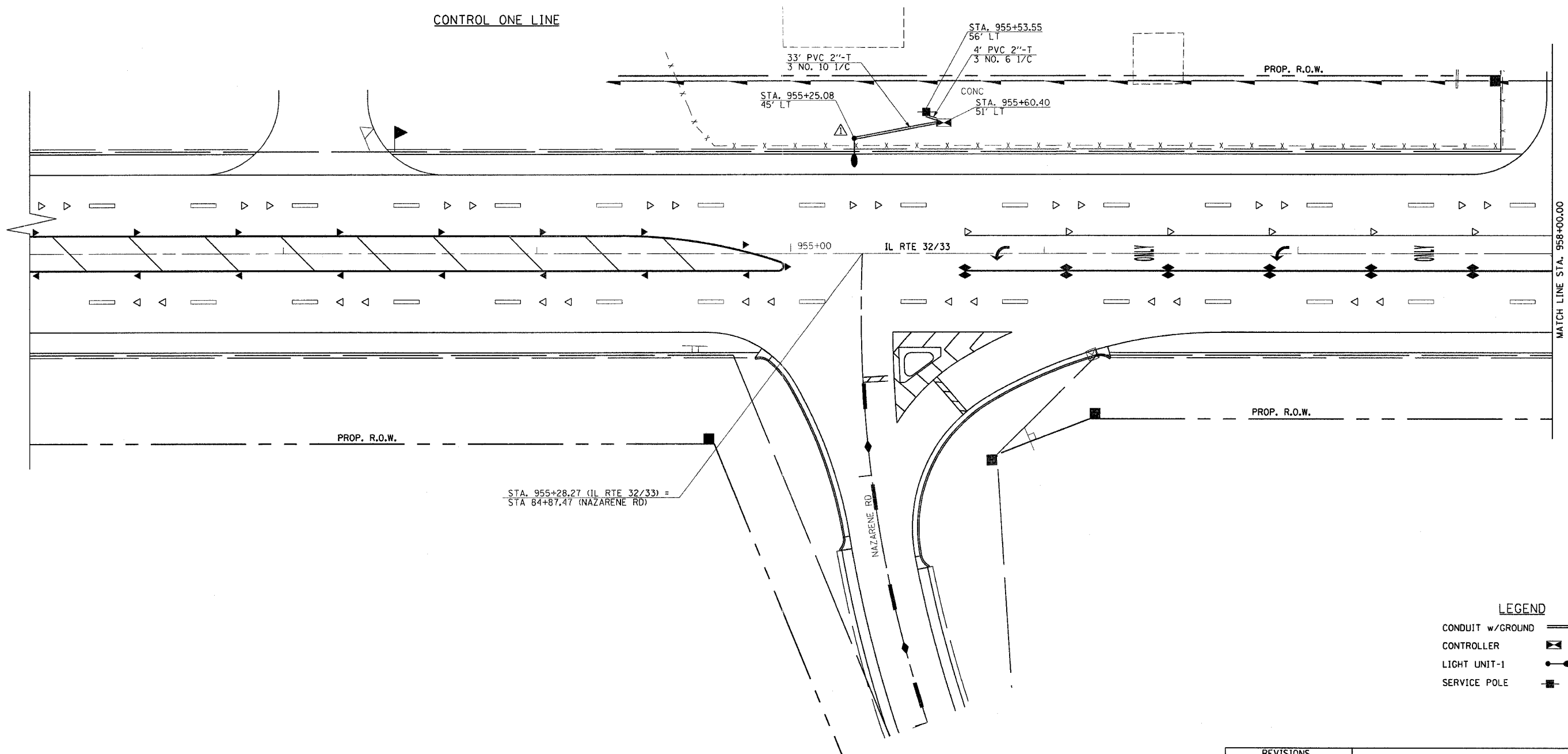
LIGHT/CABLE LAYOUT
