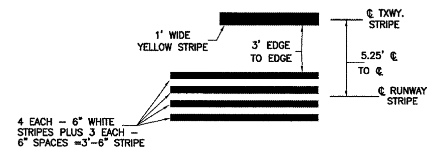
DETAIL D RUNWAY C / TAXIWAY C STRIPES
