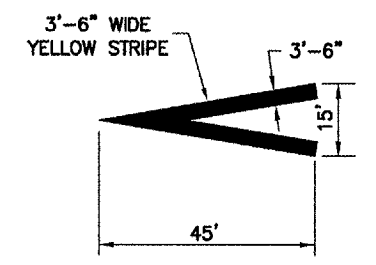
DETAIL F ARROWHEAD
