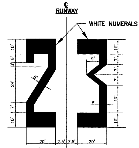
DETAIL E RUNWAY NUMERAL
