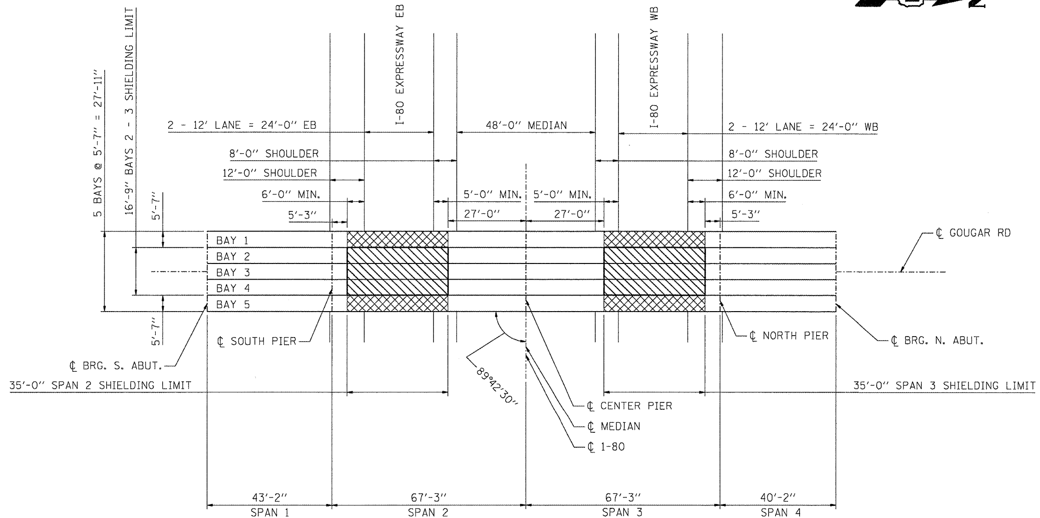
FRAMING PLAN
