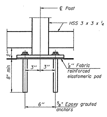
ANCHOR BOLT DETAILS
