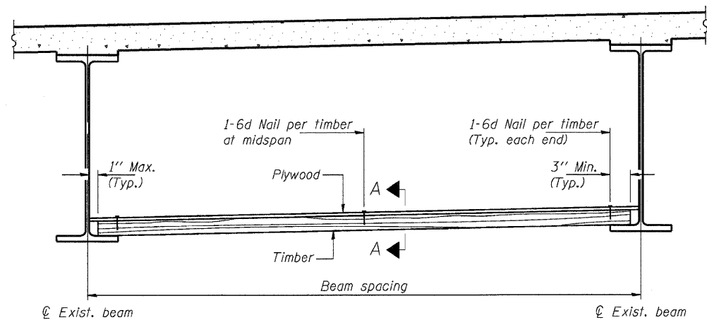
STEEL BEAMS
