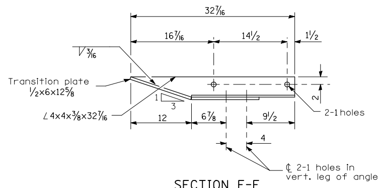
SECTION E-E
