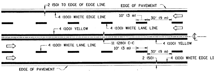
MULTI-LANE UNDIVIDED
