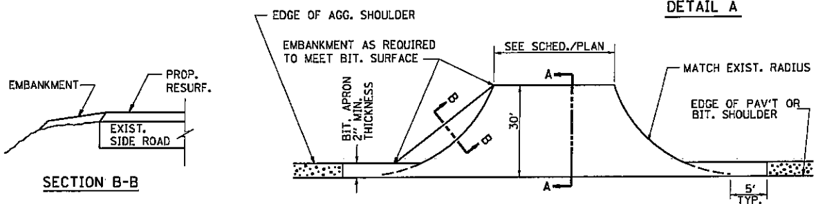
DETAIL A
