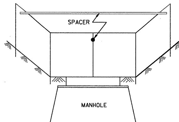
EROSION CONTROL AT OPEN GRATE MAN HOLE
