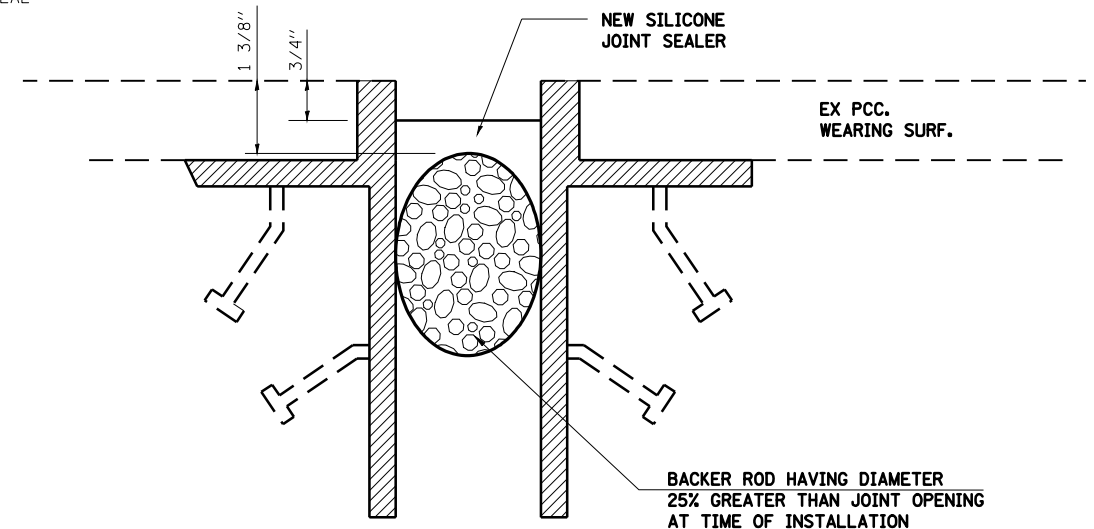
PROPOSED SILICONE JOINT SEALER DETAIL
