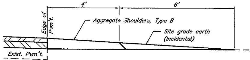
SECTION A-A FIELD ENTRANCE (Est. No. = 12)
