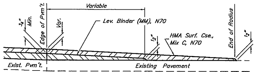
SECTION A-A SIDE ROAD (Est. No. = 11)
