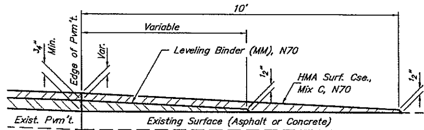
SECTION A-A PRIVATE ENTRANCE - ASPHALT (Est. No. = 6)
