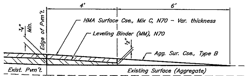
SECTION A-A PRIVATE ENTRANCE - AGGREGATE (Est. No. = 31)
