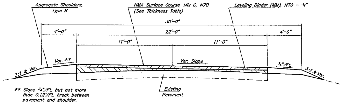
TYPICAL SECTION THRU CURVES NOTE: Section shown for right curve. Reverse for left curve.
