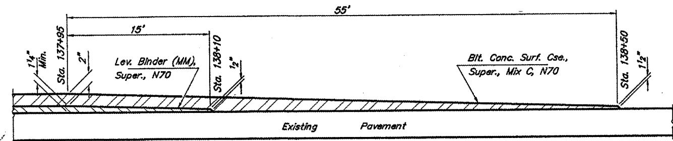
ENDING TAPER
