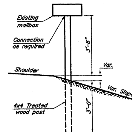
MAILBOX POST INSTALLATION DETAIL
