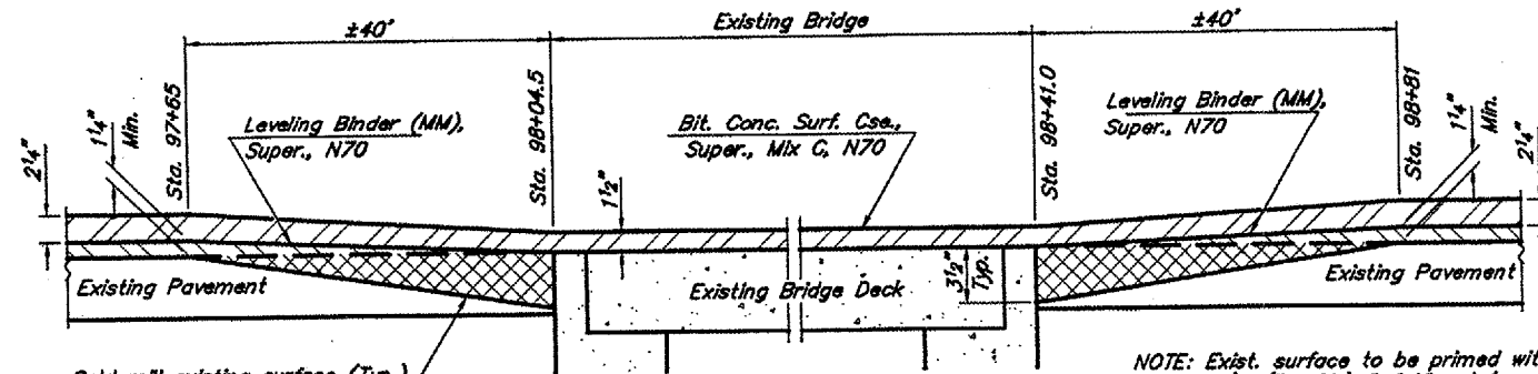
BRIDGE PAVING DETAIL - STATION 98+23
