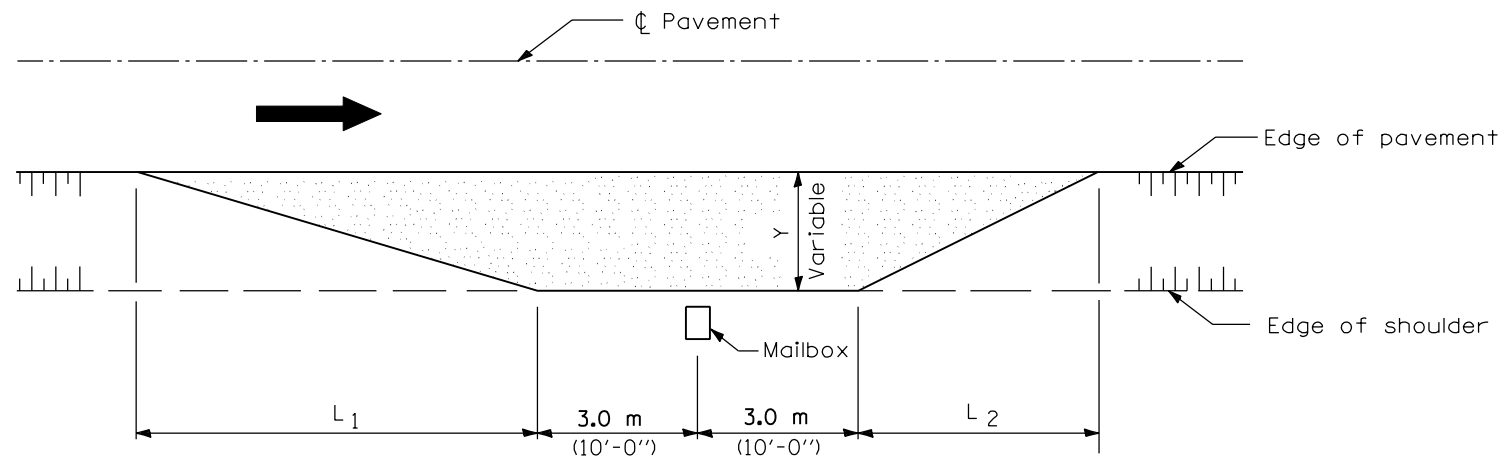
TYPICAL APPLICATION
