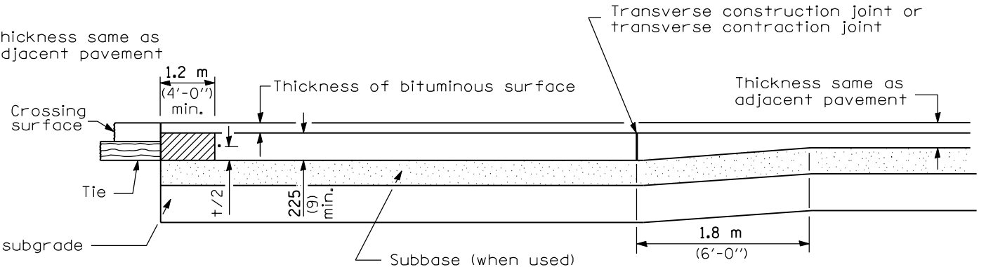
SECTION A-A (FOR PCC BASE COURSE WITH BITUMINOUS SURFACE)
