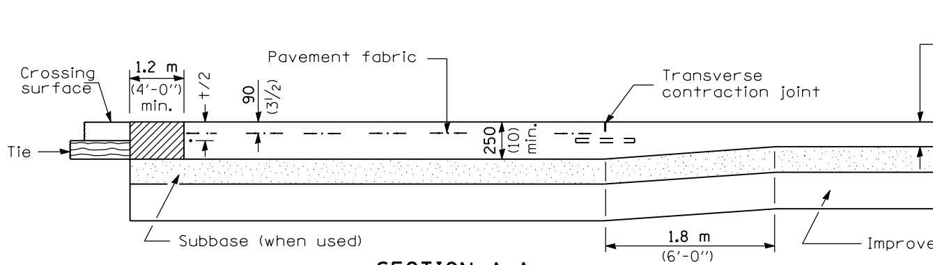
SECTION A-A (FOR PCC PAVEMENT)
