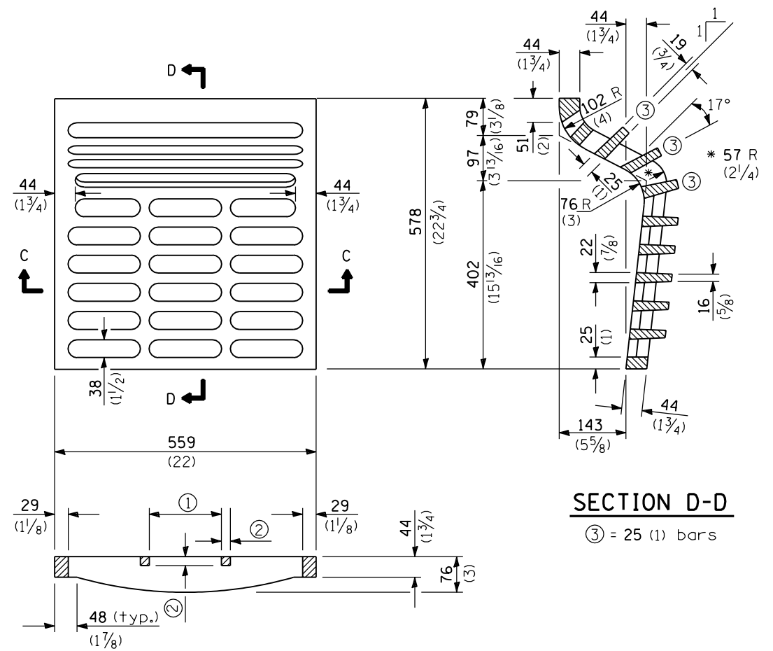
SECTION C-C
