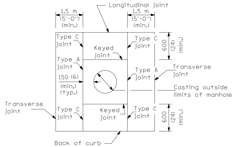
MANHOLE DETAIL Showing Joint types
