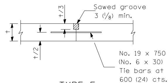
TYPE E LONGITUDINAL CONSTRUCTION JOINT
