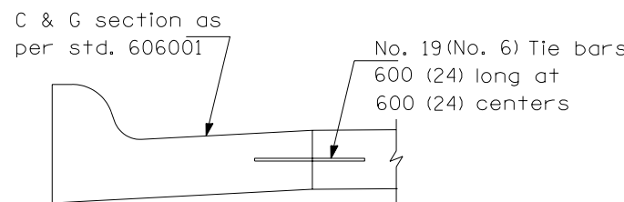
COMB. CURB & GUTTER DETAIL
