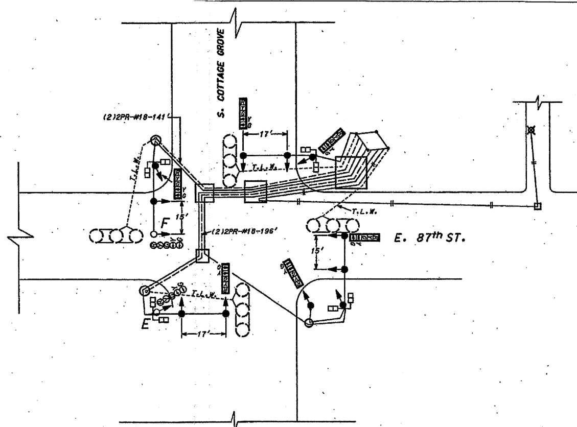
CABLE & SIGNAL PLAN NOT TO SCALE
